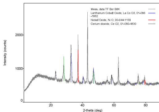
Figure 2 Diffractogram of the anode material
