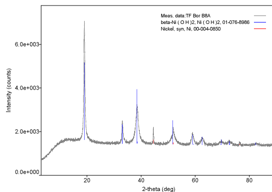
Figure 3 Diffractogram of cathode material
