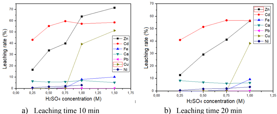
Figure 2 - Leaching rate depending on the concentration of H 2 SO 4 at a leaching time of 10 min and 20 min (leaching reagent 0.25-1.5M H 2 SO 4 , pulp density 20%, mixing speed 750 rpm, ambient temperature, without oxidant addition)
